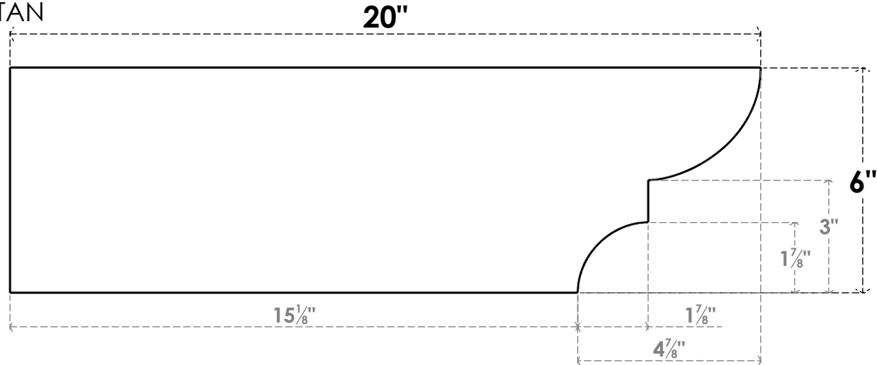
SIDE PROFILE
